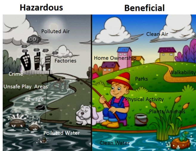
Figure 1. Conceptual environmental quality—hazardous and beneficial aspects.
